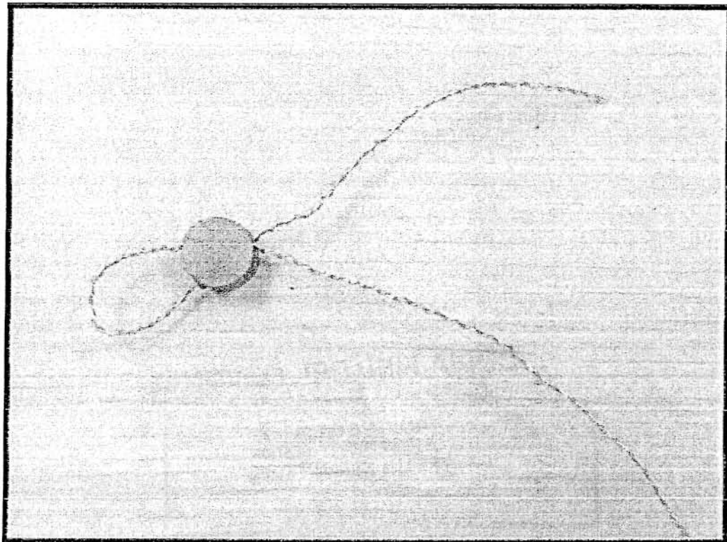
G30 Lead sealing with wire
