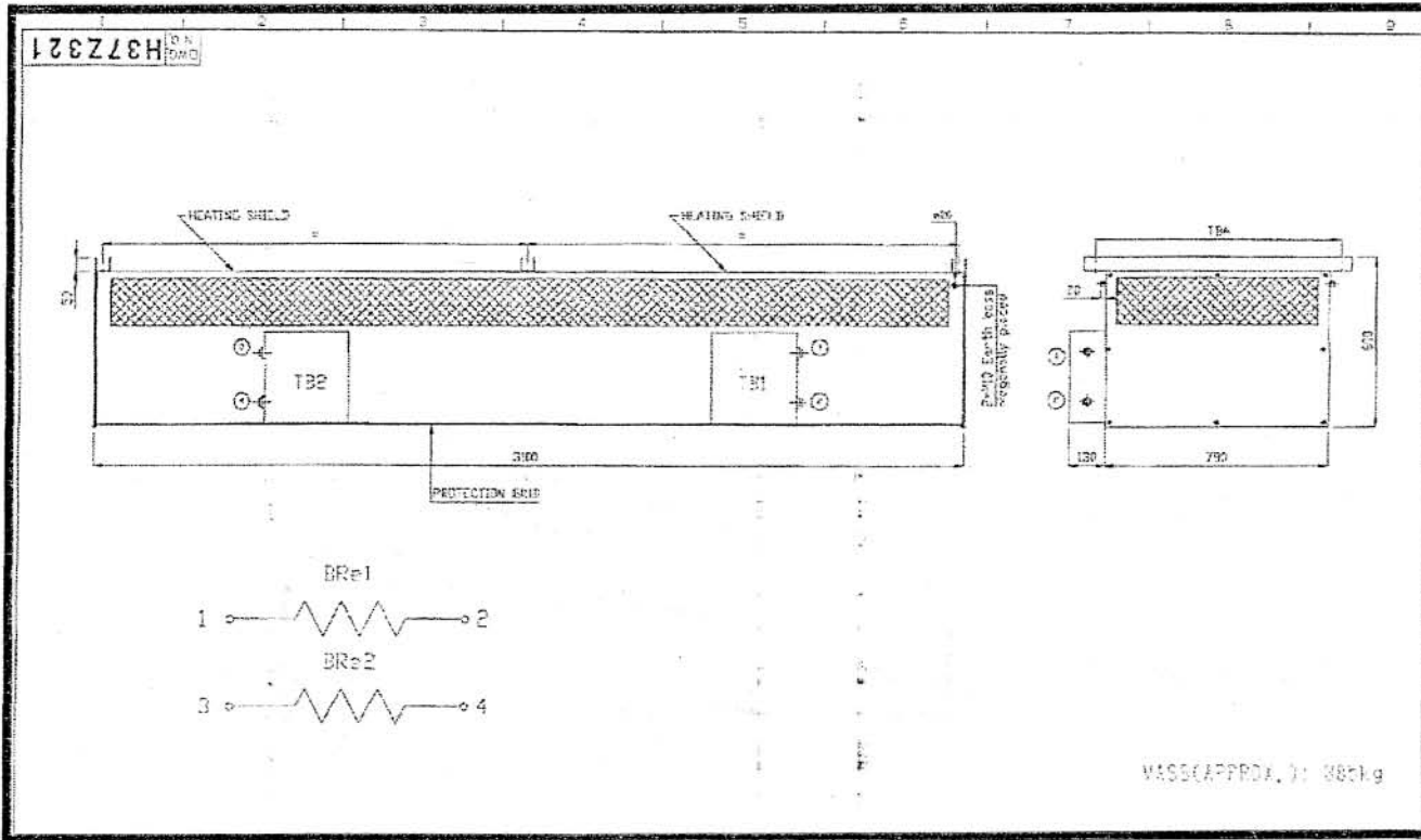
G91 Braking resistor
