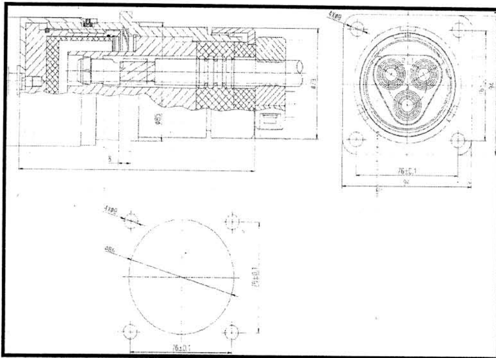
G92 Workshop power supply socket
