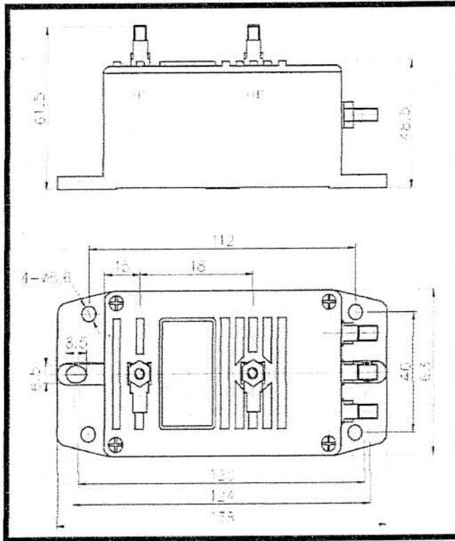
G126 Voltage sensor
