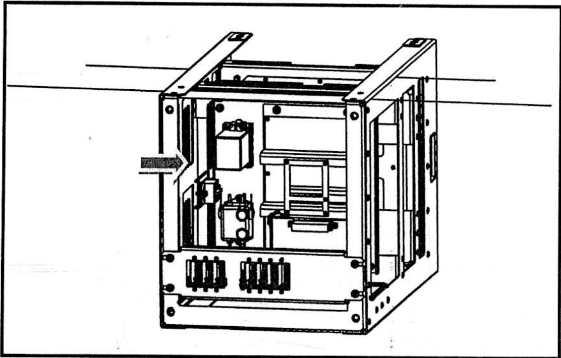
G110 Relay module for BCG
